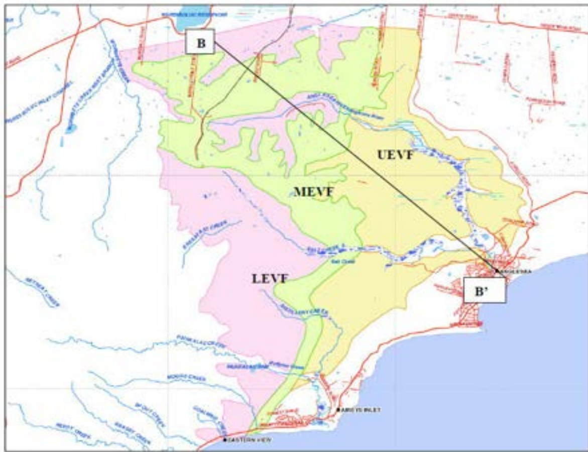
Figure 1.1. Jan Juc GMA interpreted aquifer outcrop (GHD 2019)
