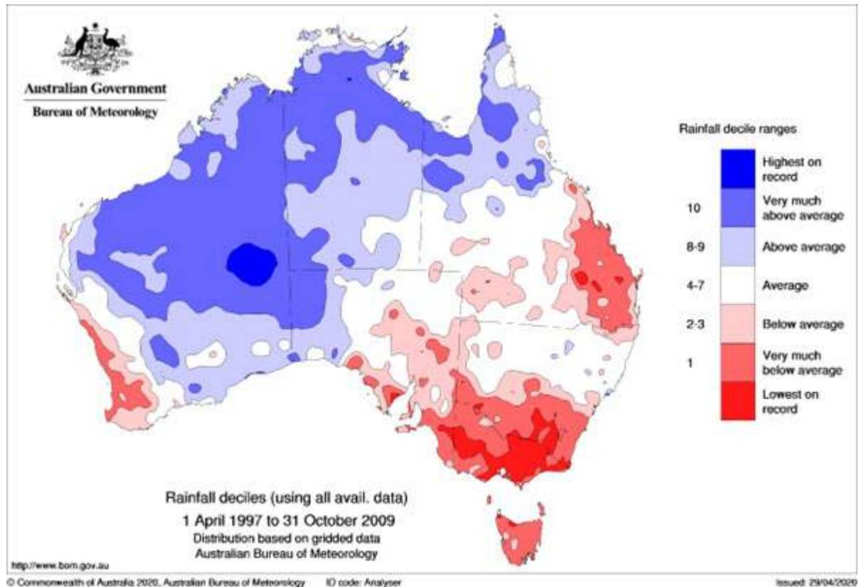
Figure 4 Rainfall Deciles for the Millennium Drought (1997 – 2009) (BoM, 2020)
