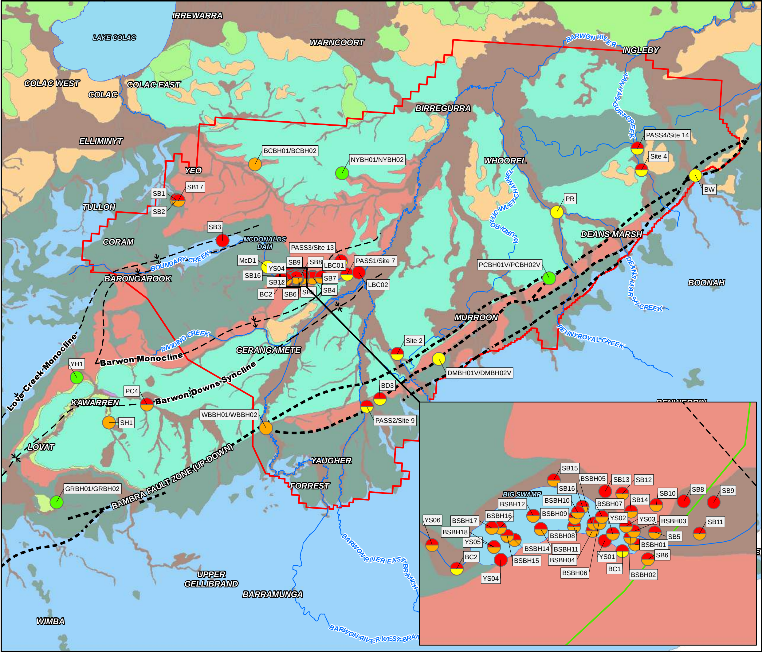
ACID SULFATE SOILS DISTRIBUTION Hydrogeological Assessment - Barwon Downs Sub-basin Barwon Downs Sub-basin Area Barwon Water Figure F21
