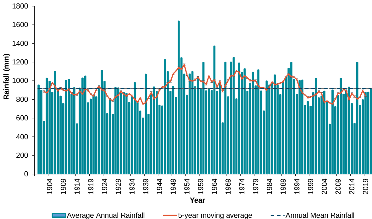
Figure 5 Average Annual Rainfall from nine rainfall station sites
